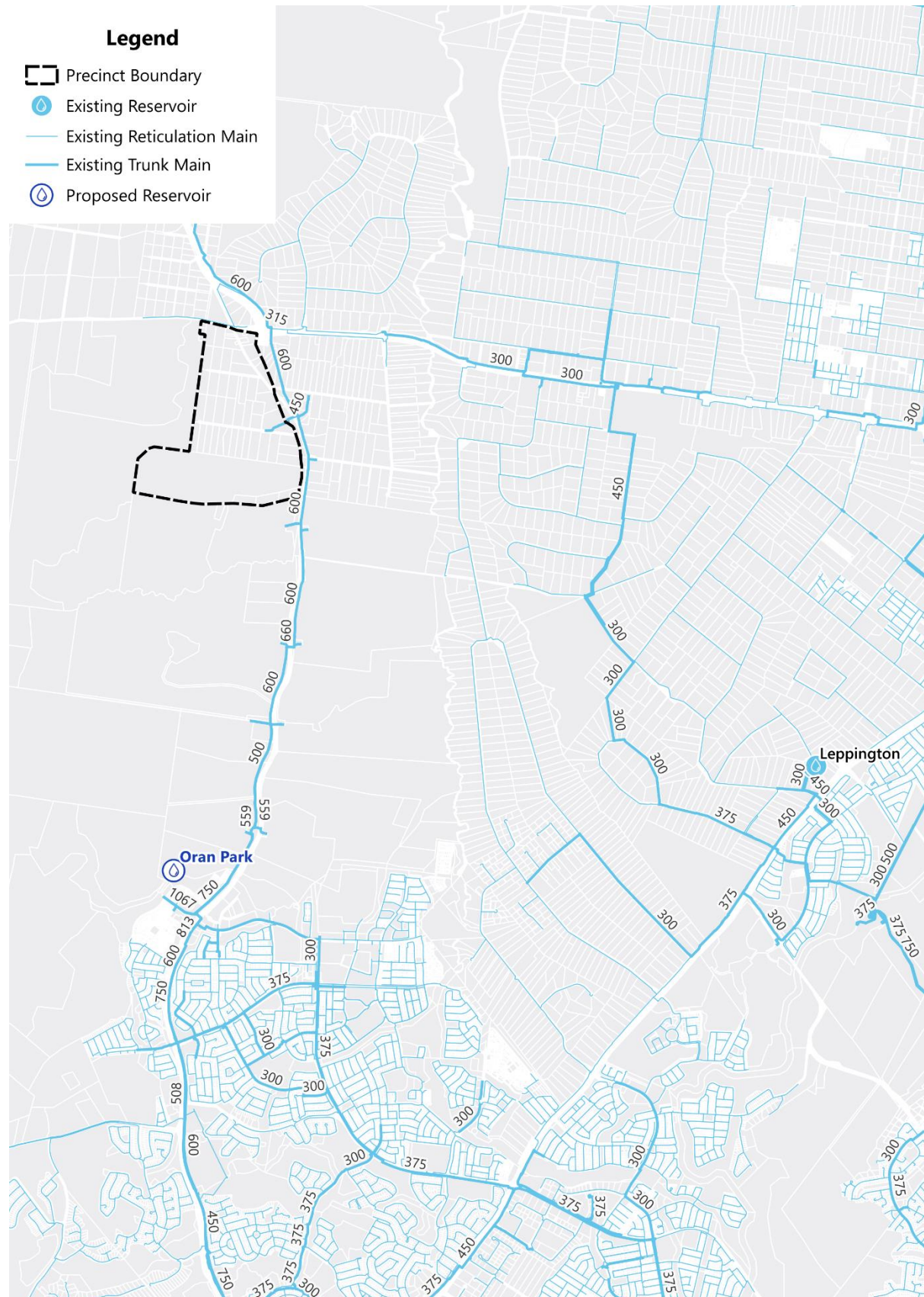
Figure 5 - Existing Potable Water Network
