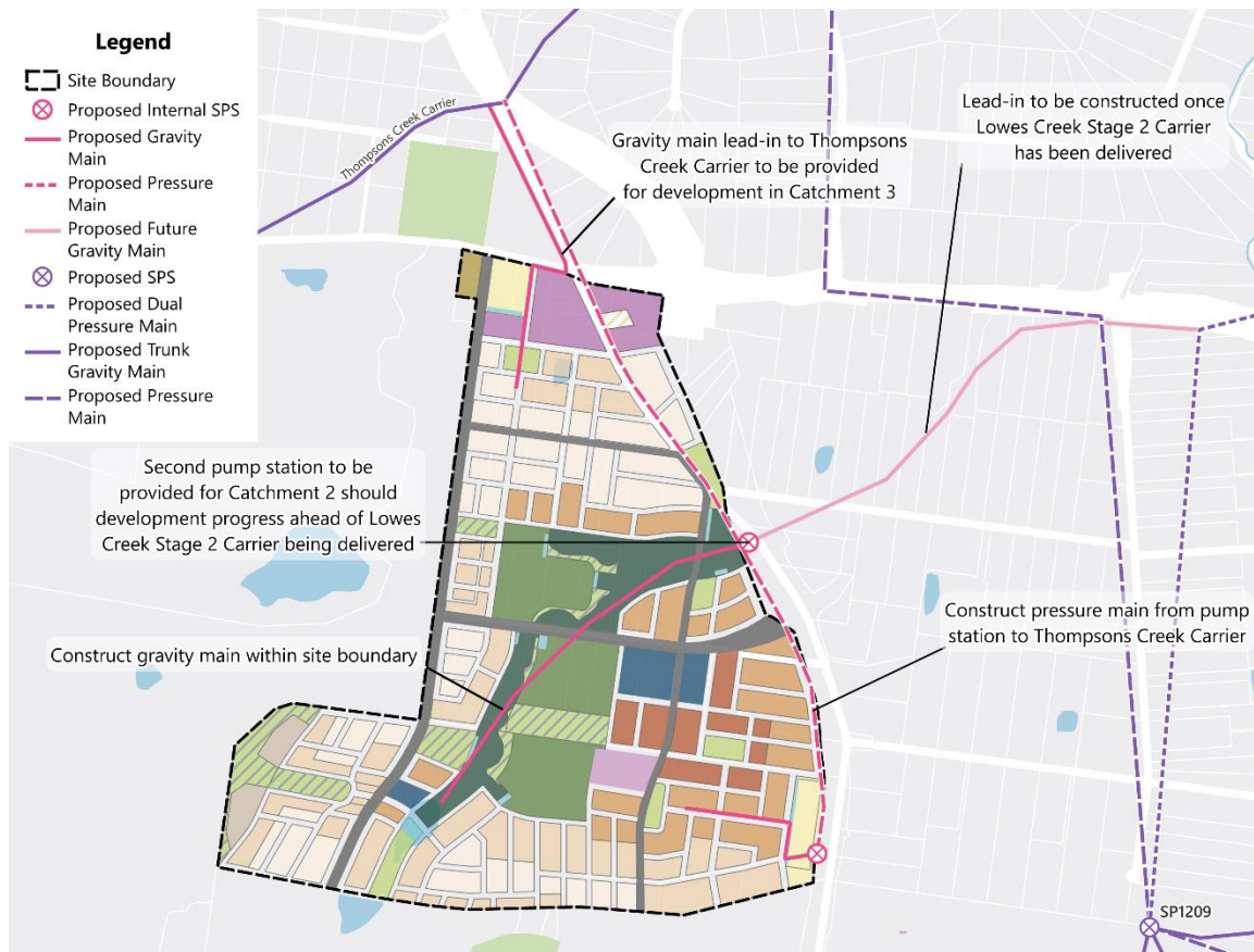
Figure 10 - Sewer Option 1
