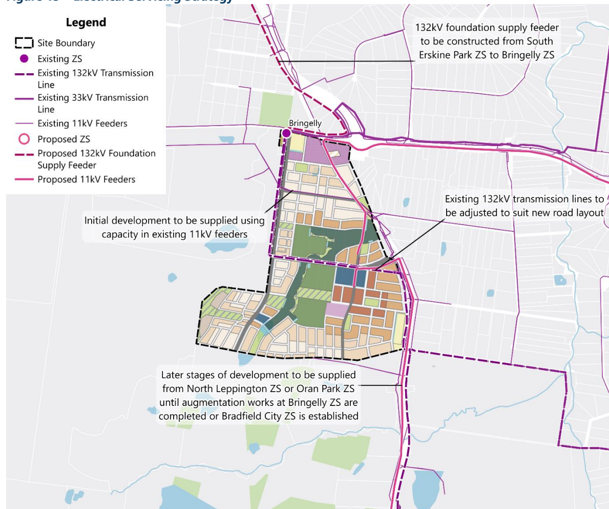
Figure 13 – Electrical Servicing Strategy
